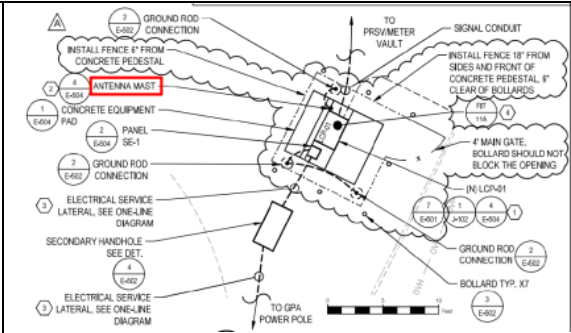
1.3 Larson Road (Please see reference drawing sheet no. 3/E-140)
