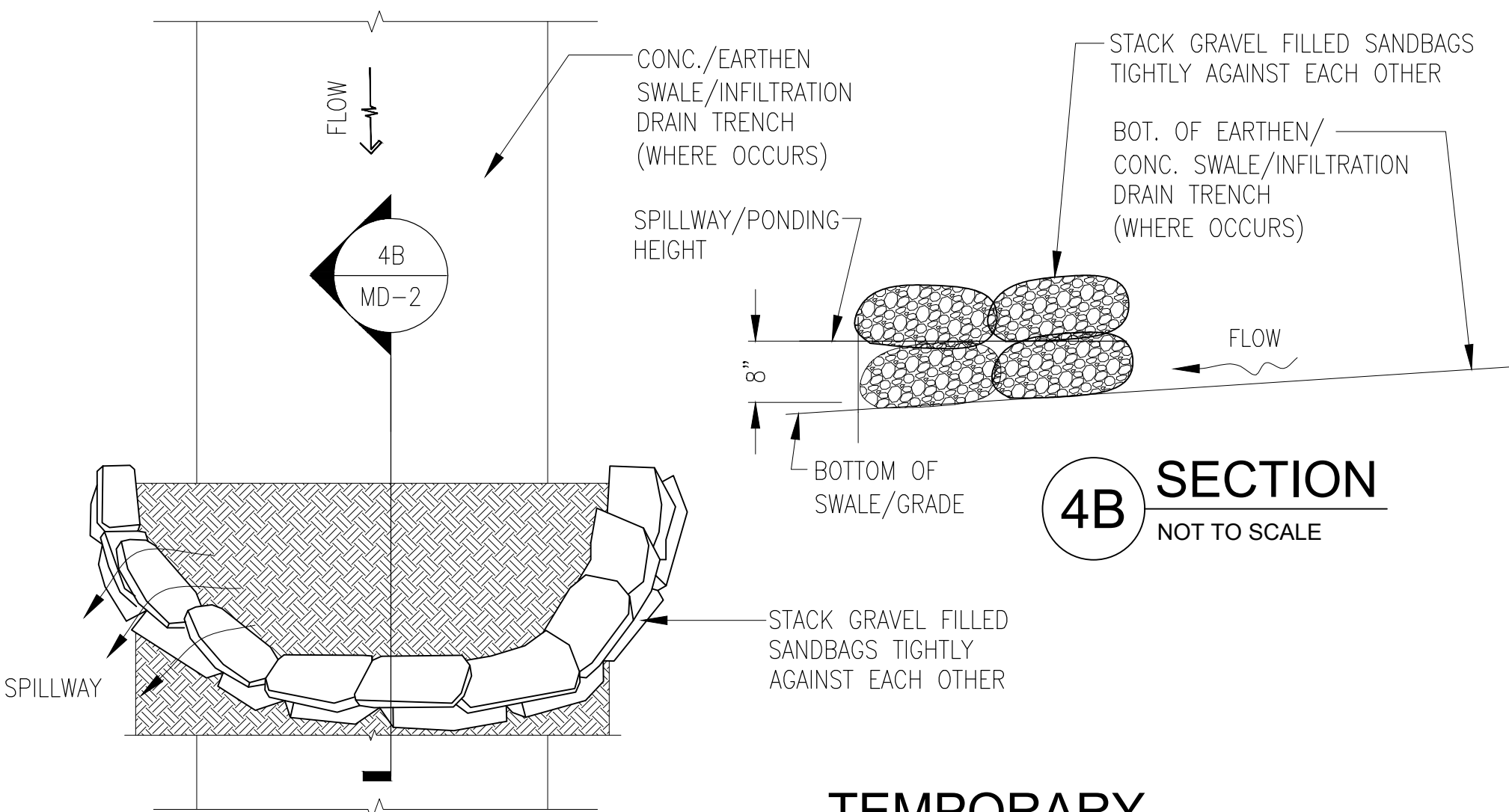
4 TEMPORARY SAND BAGS DETAIL NOT TO SCALE
