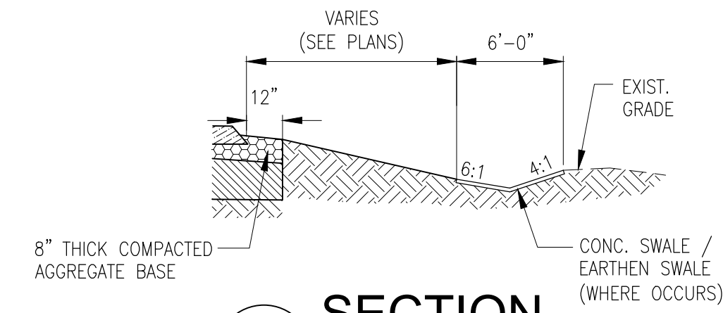
1C SECTION NOT TO SCALE
