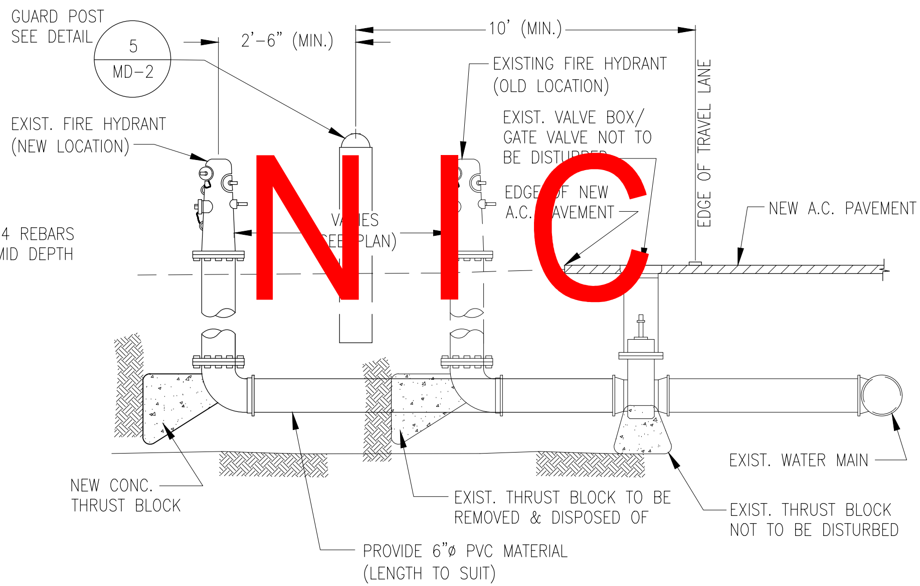
3 FIRE HYDRANT RELOCATION DETAIL NOT TO SCALE
