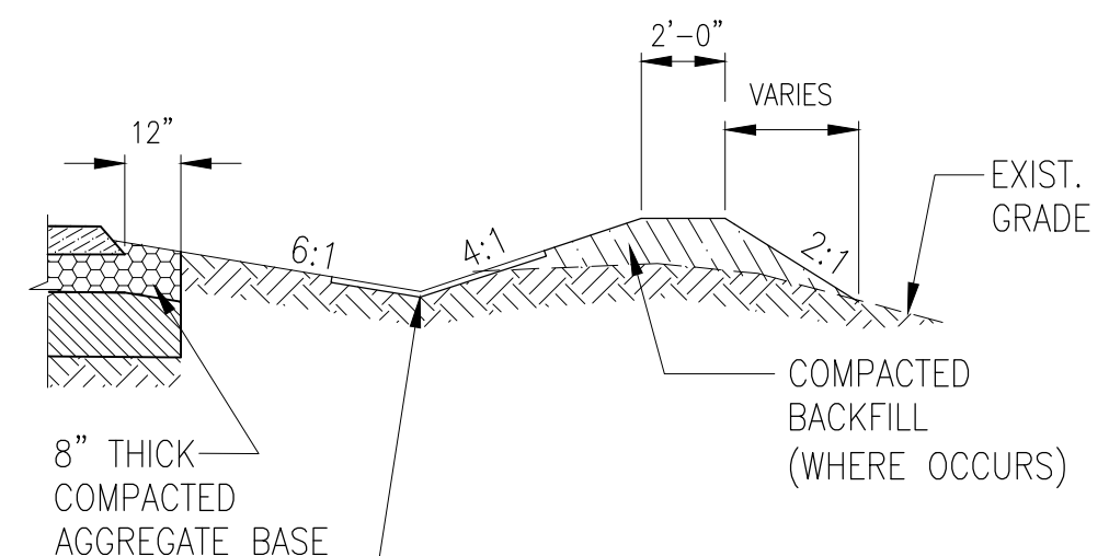
1A SECTION NOT TO SCALE
