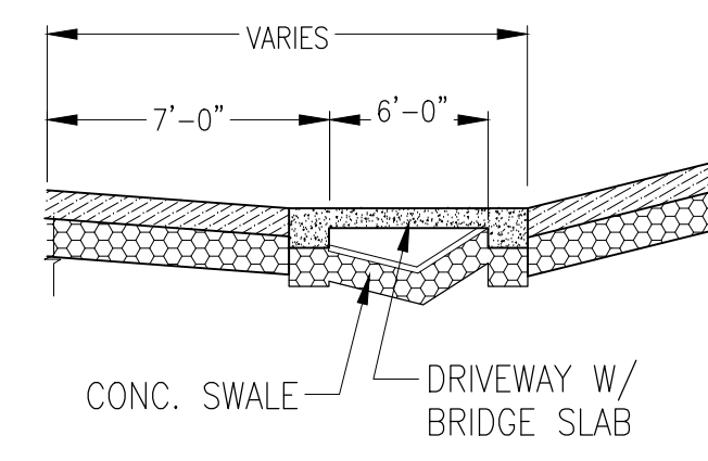
2A SECTION NOT TO SCALE
