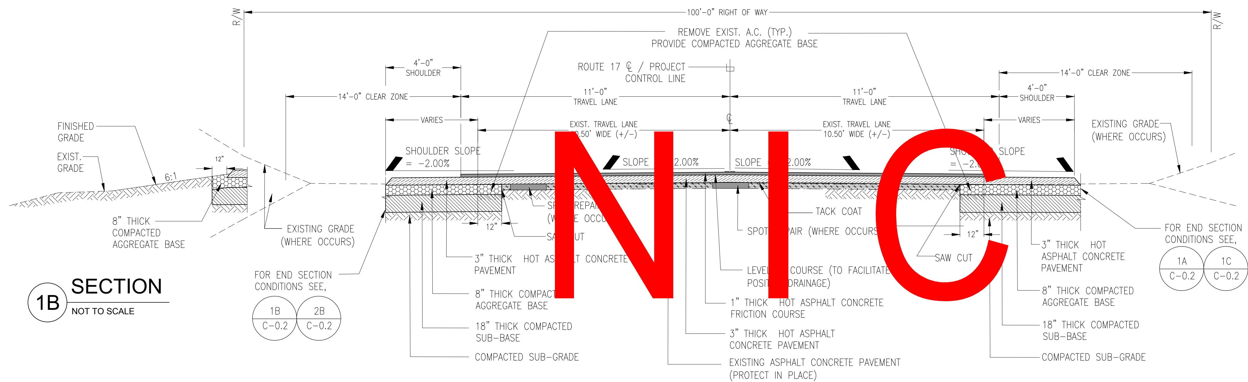
1 TYPICAL ROAD RESURFACING SECTION @ NORMAL CROWN SECTION NOT TO SCALE (STA. 28+00 TO STA. 29+00)
