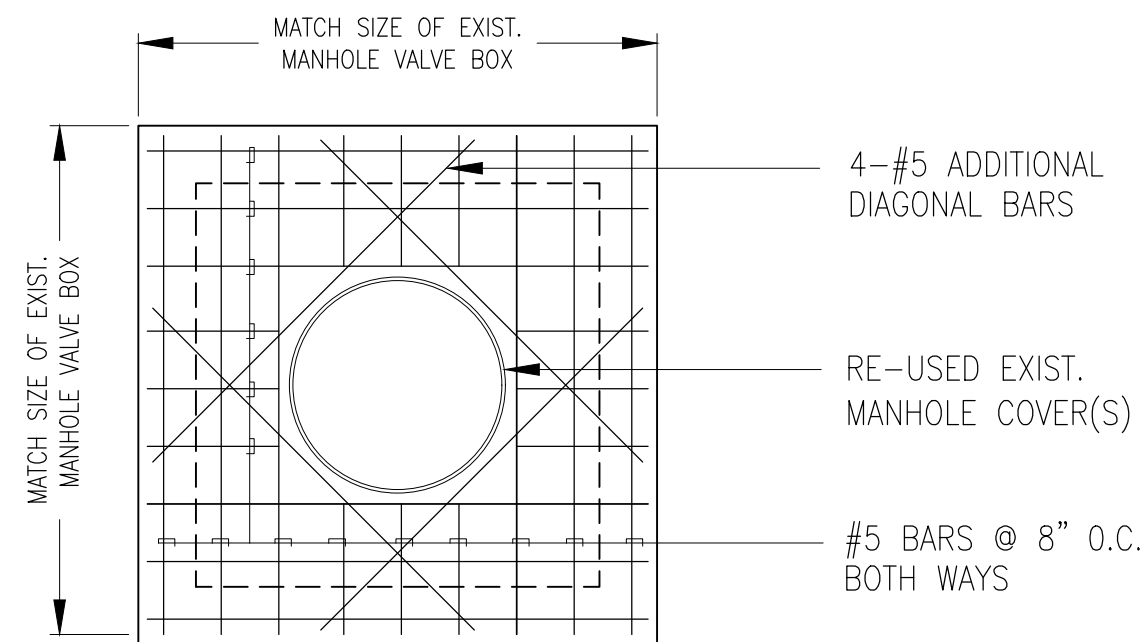
7B PLAN NOT TO SCALE
