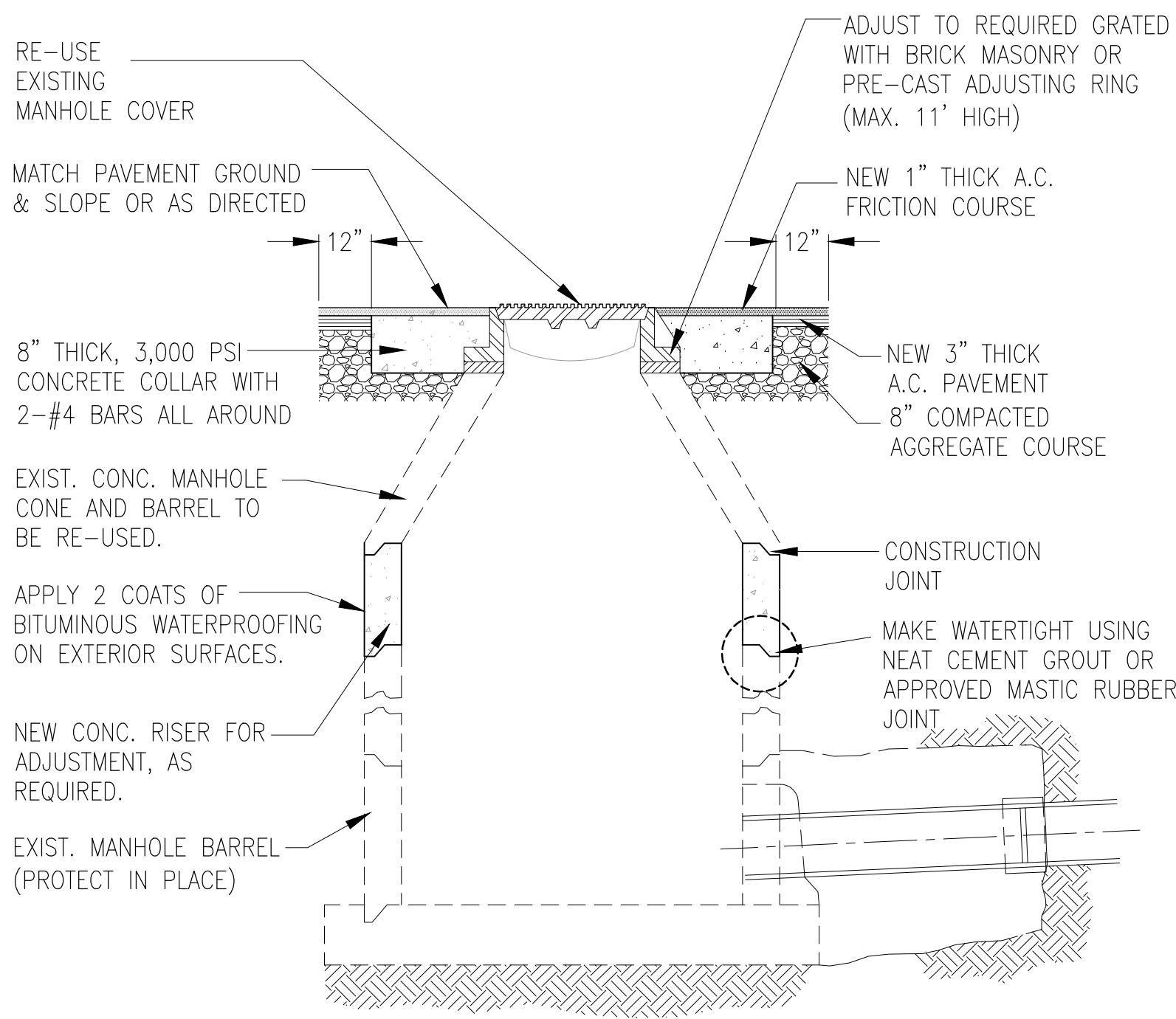
8 SEWER MANHOLE ADJUSTMENT DETAIL NOT TO SCALE
