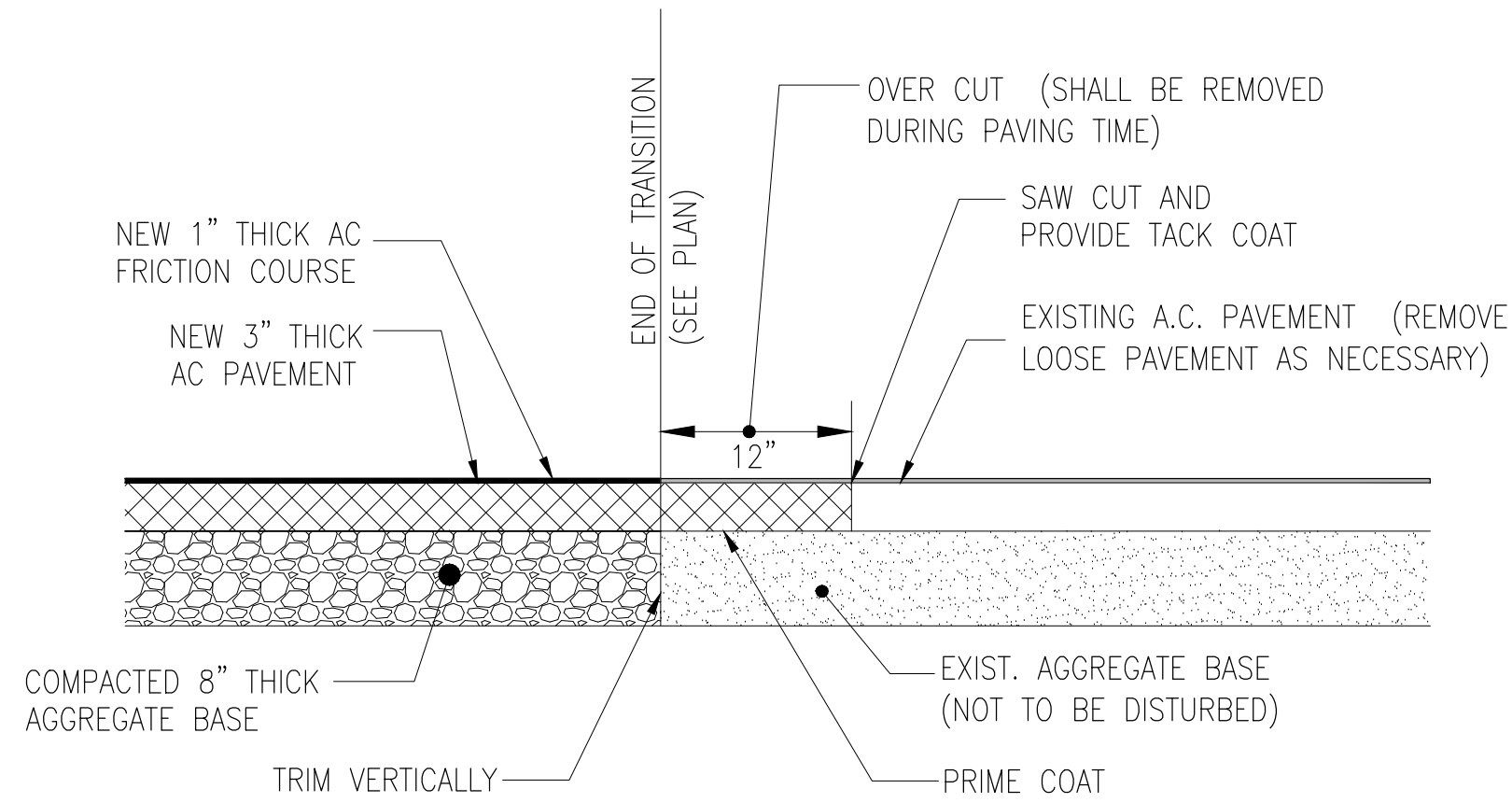
1 CONNECTION BETWEEN NEW A.C. PAVEMENT AND EXISTING A.C. PAVEMENT NOT TO SCALE
